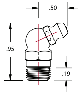
1/8" PTF SAE SPL SHORT
