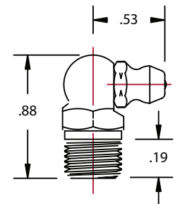
1/8" SAE SPL SHORT
