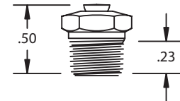
1/8" BSPT RELIEF FITTING
