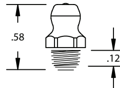
1/4"-28 SPECIAL TAPER THD. (Recommended hole size-.230 to .235")
