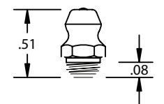
1/4"-28 SPECIAL TAPER THD. (Recommended hole size-.230 to .235")
