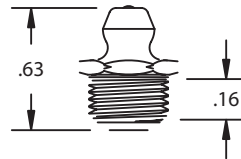
1/8" PTF SAE SPL EXTRA SHORT
