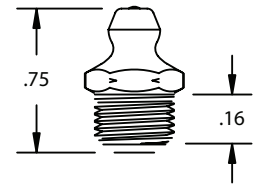
1/8" SAE SPL EXTRA SHORT
